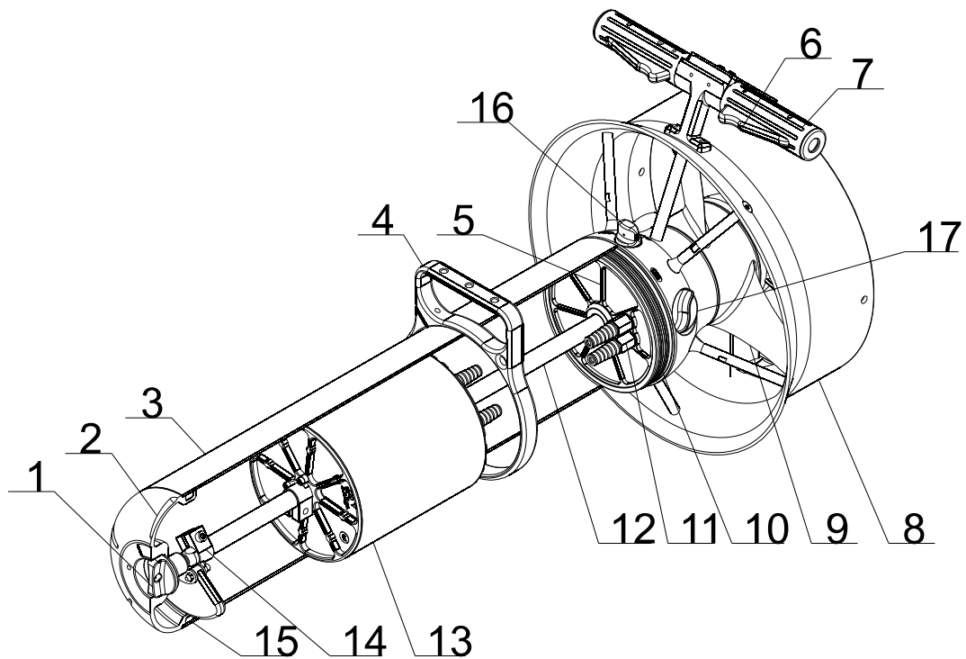
Drawing 1. Summary of basic scooter components
