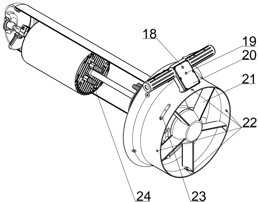
Drawing 2. Summary of basic scooter components
